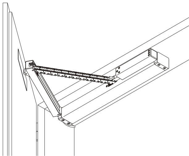
DDS 50/500 in Türzarge montiert / mounted in the case of door
